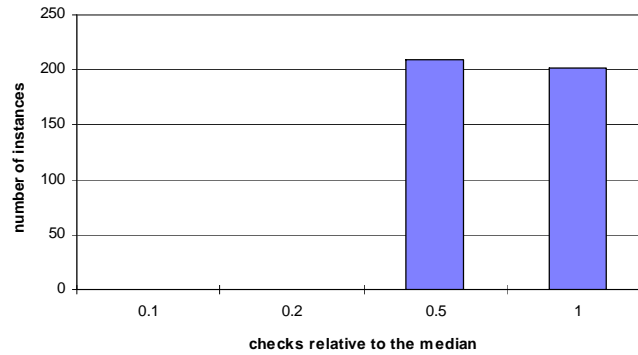
Figure 13 - Search cost for problems where no switch was predicted for BM+MWO (total of 411 instances)
