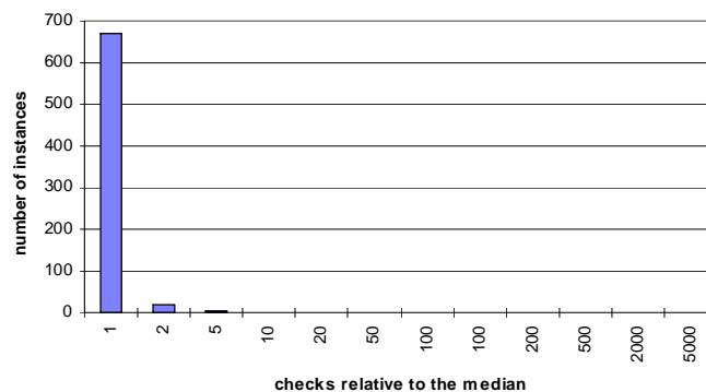
Figure 12 - Cost to predict a switch for BMCBJ+MWO (total of 693 instances)
