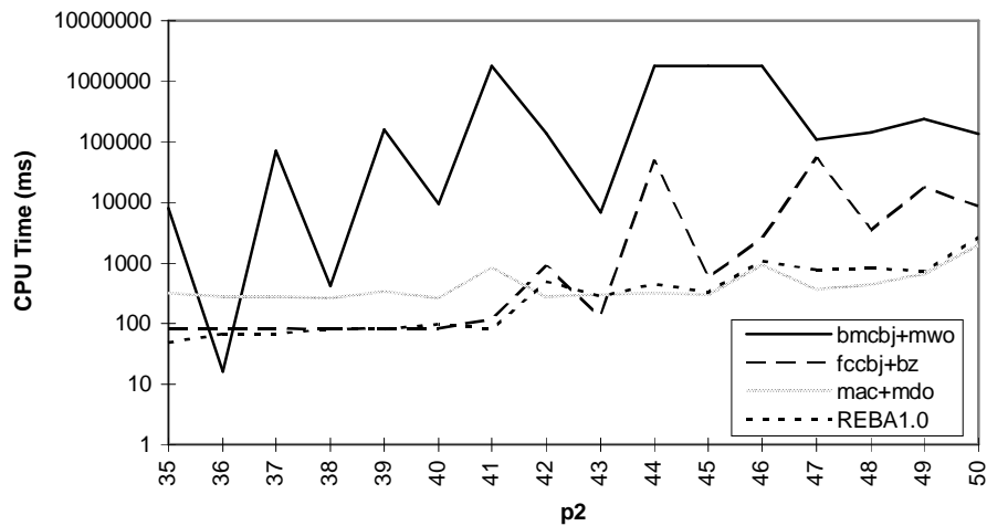
Figure 6 - worst case performance on 50 variable problems in terms of cpu time
