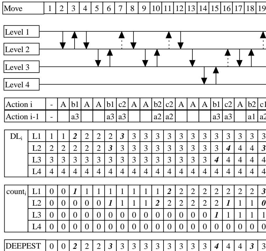
Figure 2 - Example search
