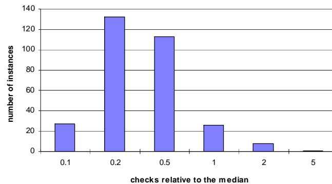
Figure 14 - Search cost for problems where no switch was predicted for BMCBJ+MWO (total of 307 instances)
