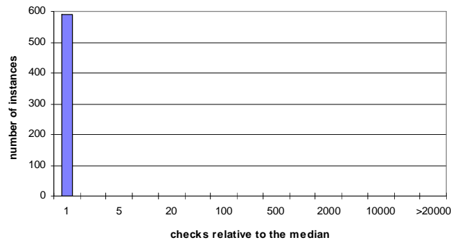
Figure 11 - Cost to predict a switch for BM+MWO (total of 589 instances)
