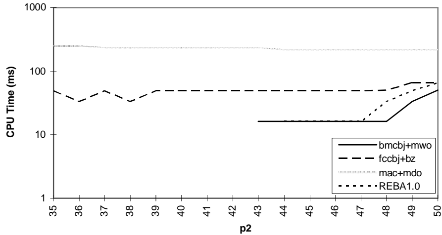
Figure 5 - median performance on 50 variable problems in terms of cpu time 9
