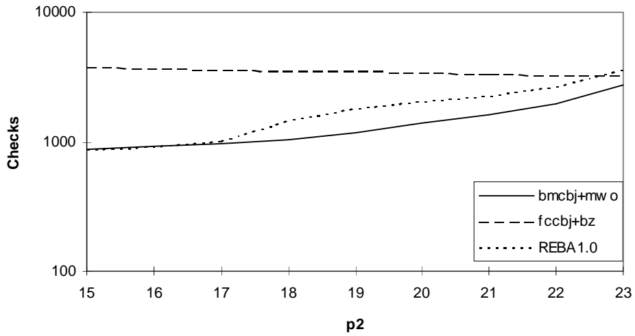
Figure A1 - median performance on 100 variable problems in terms of compatibility checks
