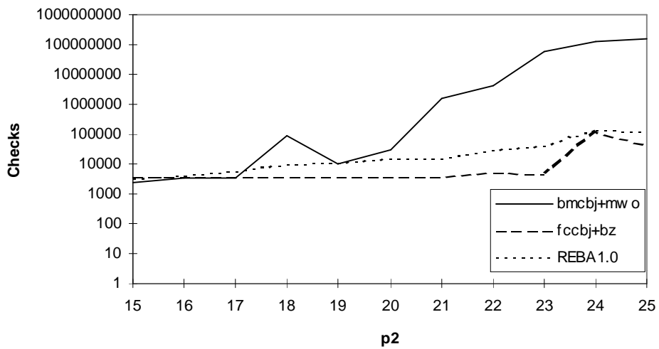
Figure A2 - worst case performance on 100 variable problems in terms of compatibility checks
