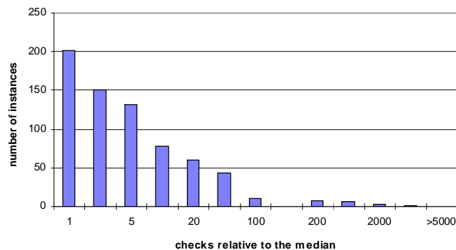
Figure 10 - Ultimate search cost for BMCBJ+MWO had a switch not been predicted (total of 693 instances)
