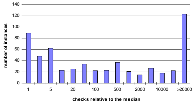
Figure 9 - Ultimate search cost for BM+MWO had a switch not been predicted (total of 589 instances)
