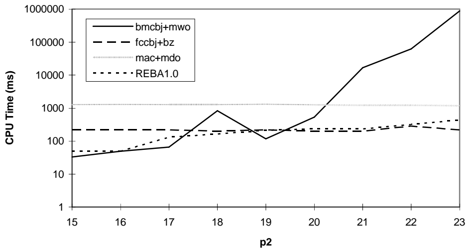
Figure A4 - worst case performance on 100 variable problems in terms of cpu time
