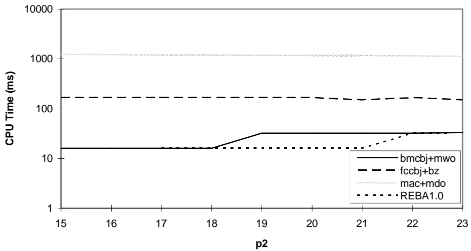
Figure A3 - median performance on 100 variable problems in terms of cpu time
